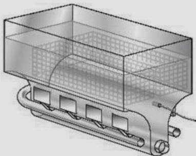
picture of gas open pot design showing cook, heat, and cold zone or sediment zone
